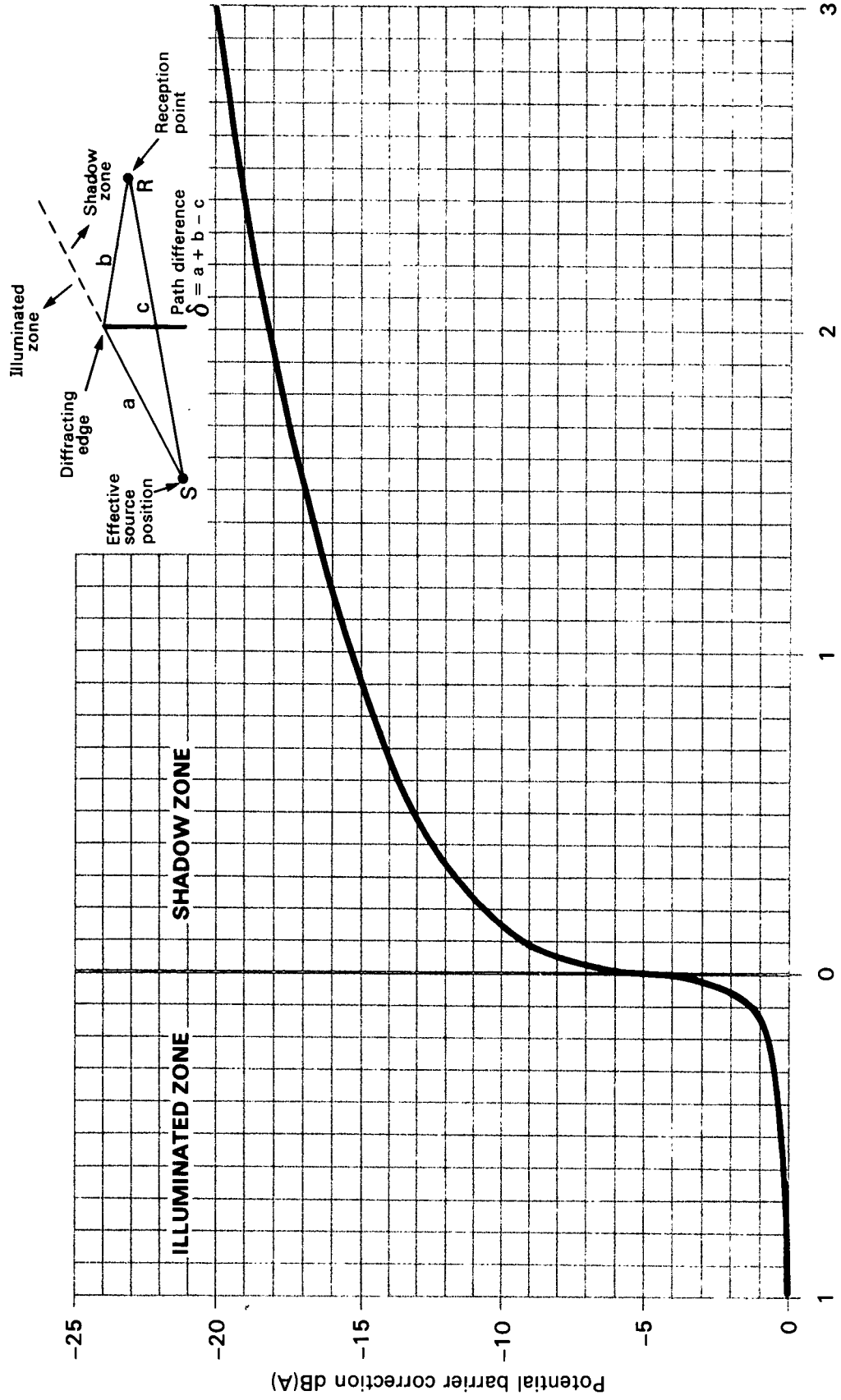
Chart 9 POTENTIAL BARRIER CORRECTION AS A FUNCTION OF PATH DIFFERENCE \delta
