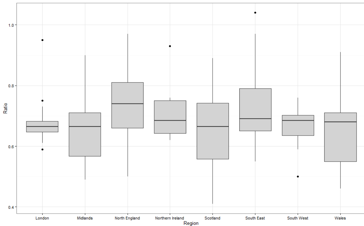
Figure B.7 – A Box and Whisker Plot showing the Spread in the Annual Average Ratio of PM_{2.5}/PM_{10} as a Function of Region for All Years
